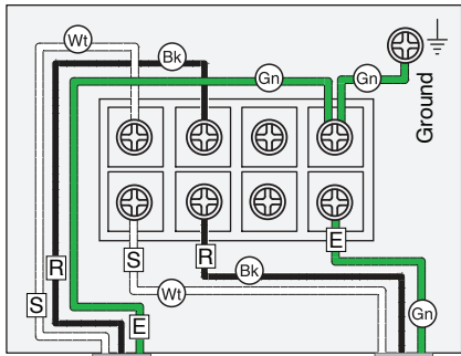
POWER SUPPLY JUNCTION BLOCK
