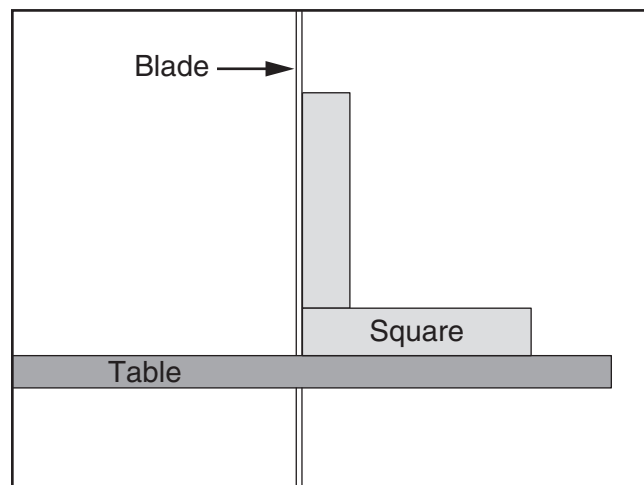
Figure 79. Squaring table to blade.
