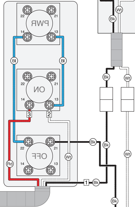
CONTROL PANEL (viewed from behind)
