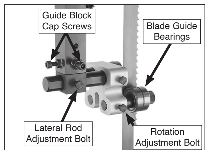
Figure 25. Rear upper blade guide controls.
