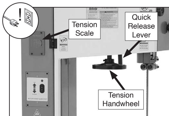
Figure 23. Blade tension controls.
