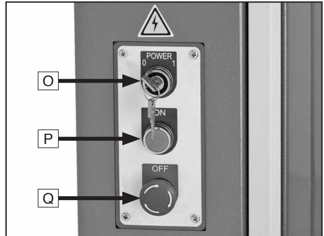
Figure 3. Control panel.
