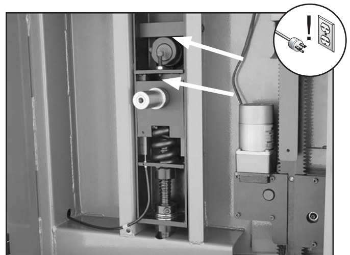
Figure 63. Tension adjustment assembly locations (top wheel removed for clarity).
