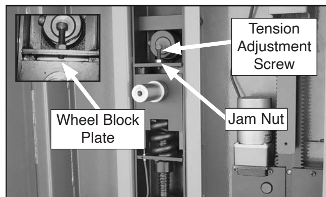
Figure 71. Quick release tension lever adjustment screw.
