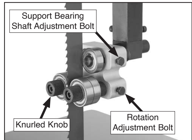
Figure 24. Front upper blade guide controls.
