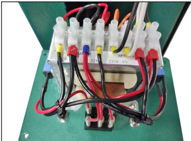
Figure 87. Guide post elevation control wiring.
