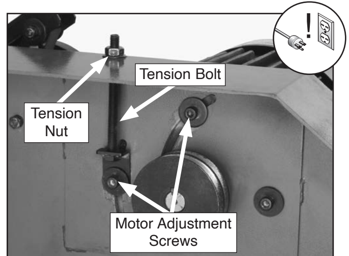
Figure 67. Motor mount bolts and tension bolt (lower wheel removed for clarity).
