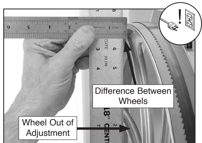
Figure 83. Determining distance needed to shim upper wheel.
