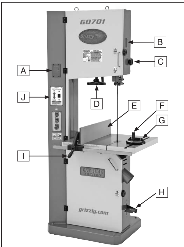
Figure 1. Front controls.
