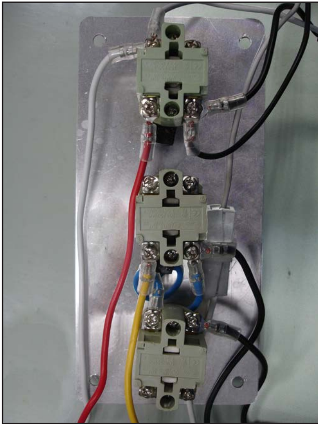
Figure 86. Control panel wiring.
