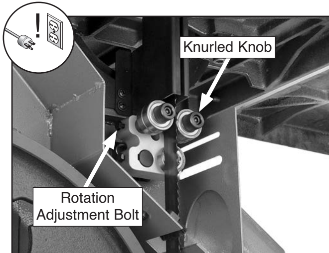
Figure 34. Front lower blade guide controls.
