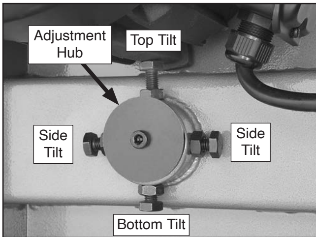
Figure 84. Lower wheel adjustment control.
