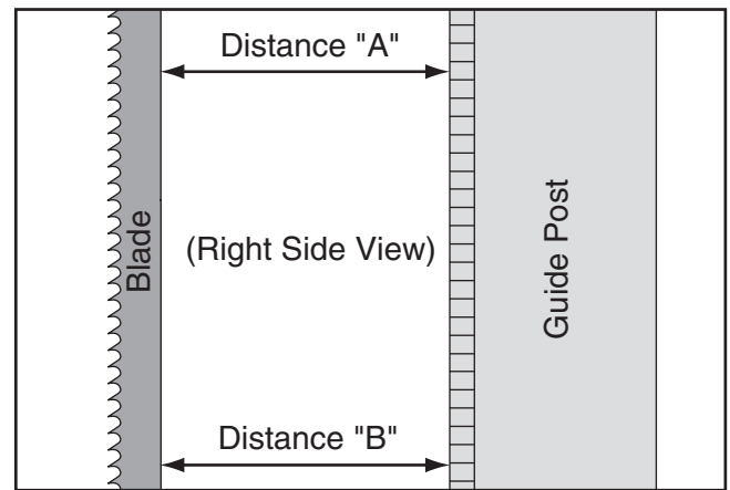
Figure 76. Example of measuring distance between rack and blade at top of guide post.
