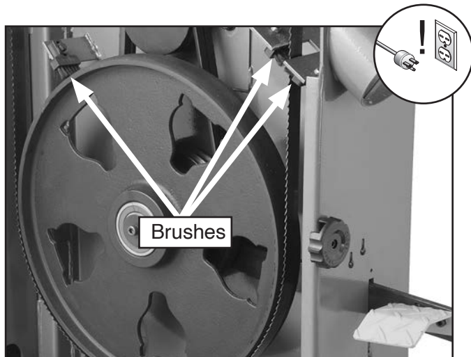
Figure 70. The wheel brush and blade brushes.
