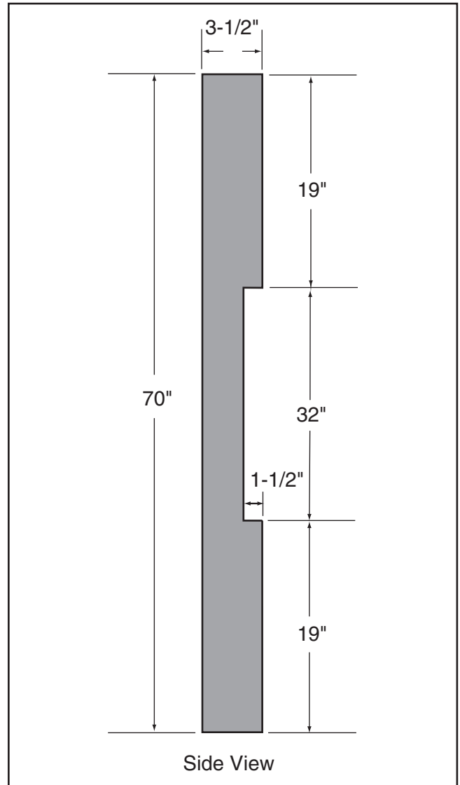
Figure 80. Dimensions of coplanarity gauge.
