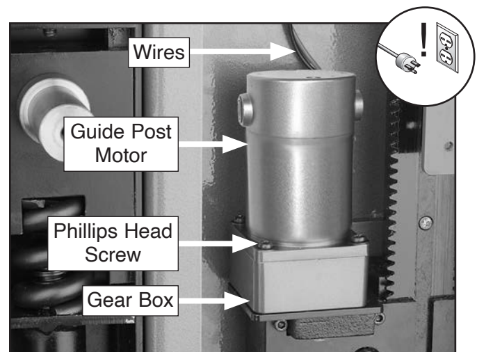
Figure 78. Location of guide post motor.
