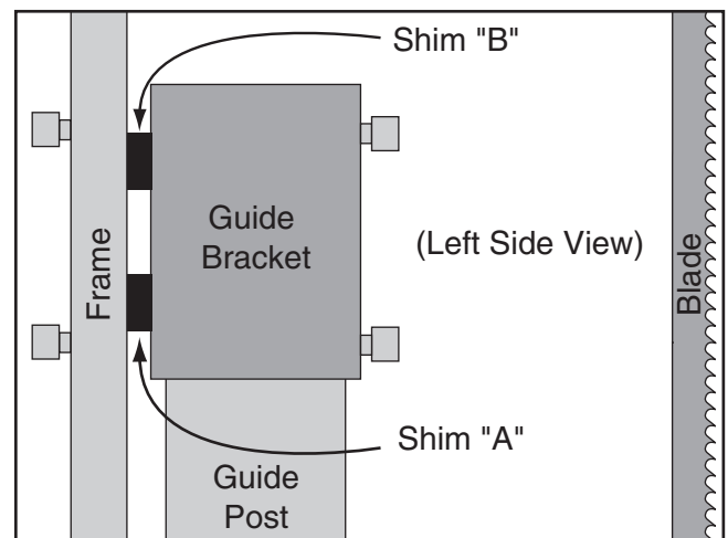
Figure 77. Location for placing shims. (Shim thickness not drawn to scale.)
