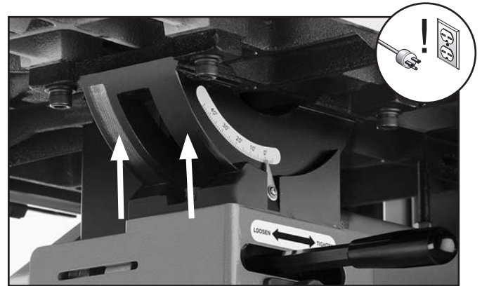
Figure 65. Trunnion lubrication location.
