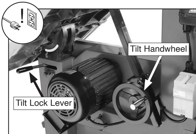
Figure 17. Table tilted up.
