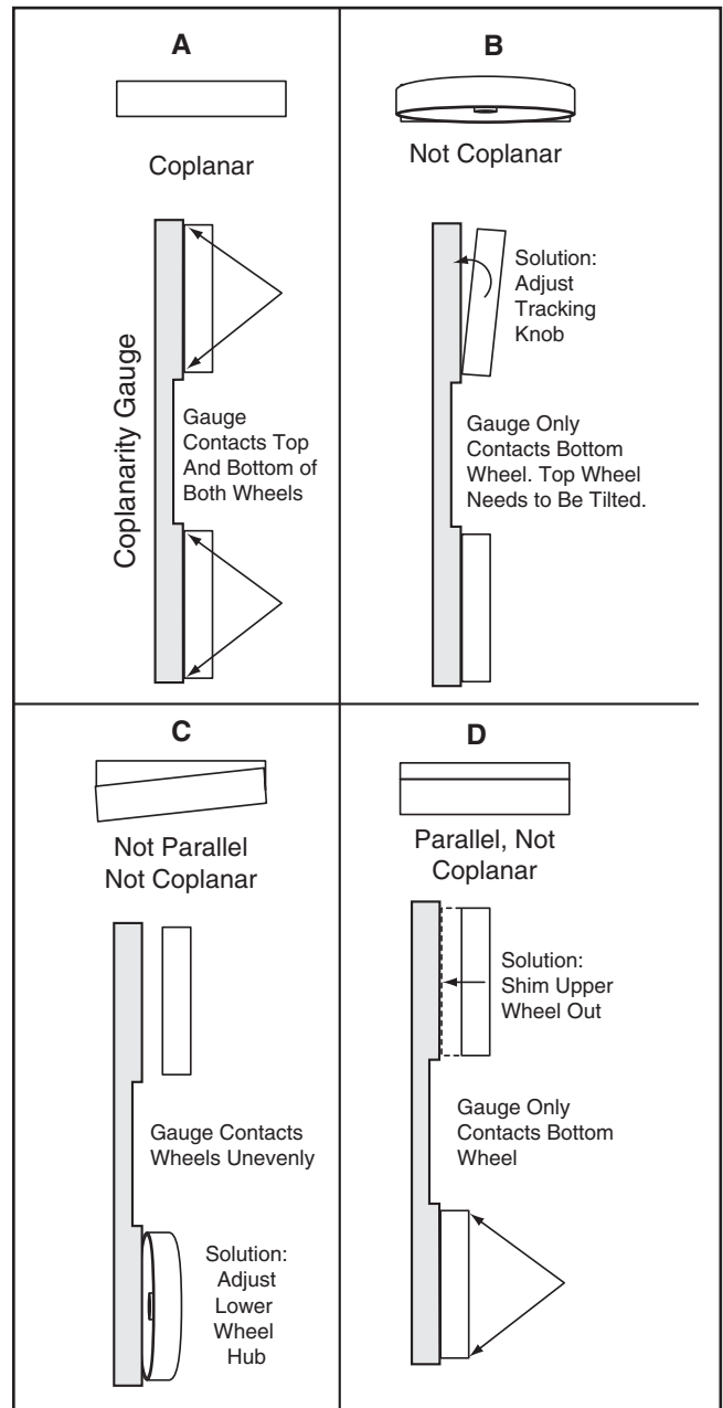
Figure 82. Coplanarity diagram.
