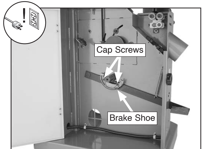
Figure 79. Brake shoe location.
