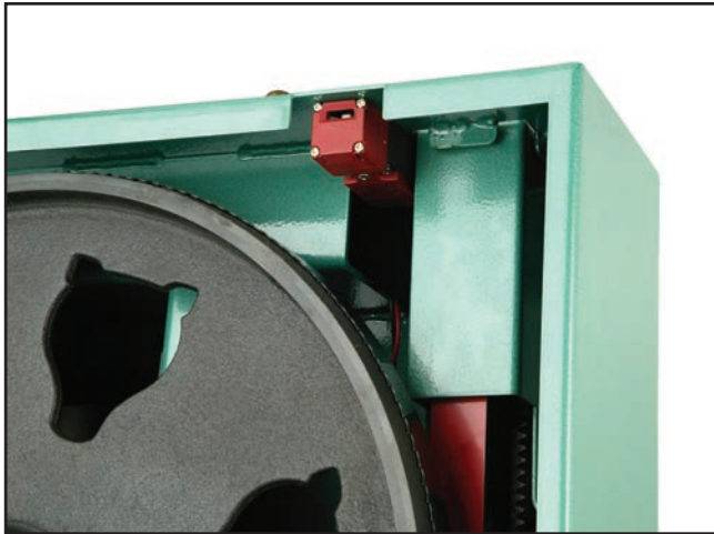
Figure 88. Upper door safety switch wiring.
