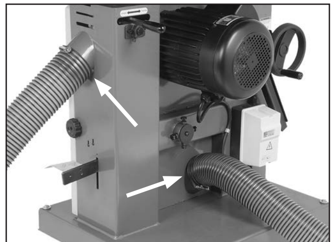
Figure 13. Dust hoses attached.
