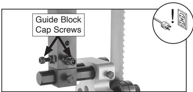
Figure 75. Guide block cap screws (blade guard removed for photo clarity).
