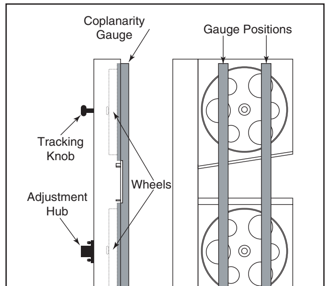
Figure 81. Checking for coplanarity.
