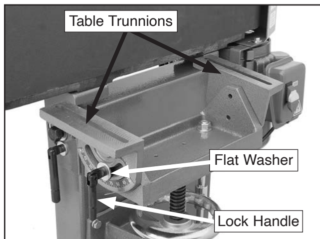
Figure 22. Table trunnions installed.
