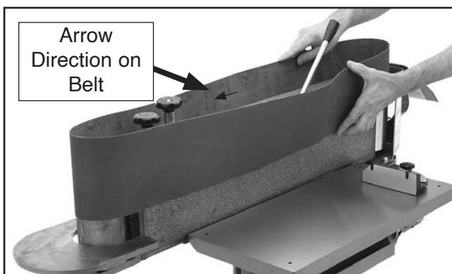
Figure 41. Installing the sanding belt.
