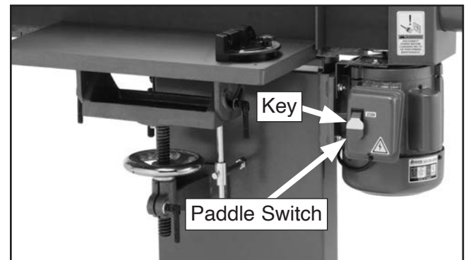
Figure 30. Paddle switch location.
