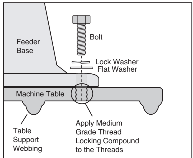
Figure 11. Direct mounting.
