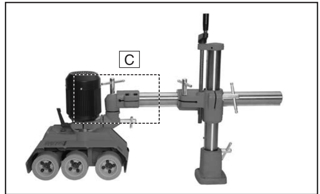
Figure 8. Assembled unit.
