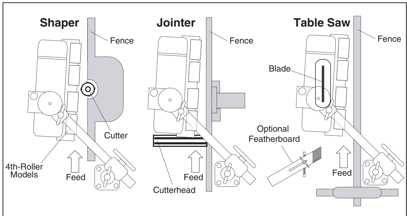
Figure 9. Typical power feeder mounting on a shaper, jointer, and table saw.
